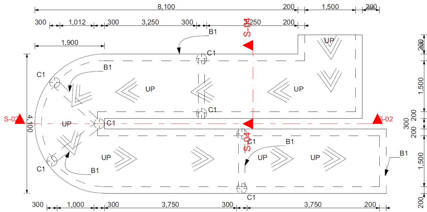
RAMP GROUND PLAN & COLUMN LAYOUT
