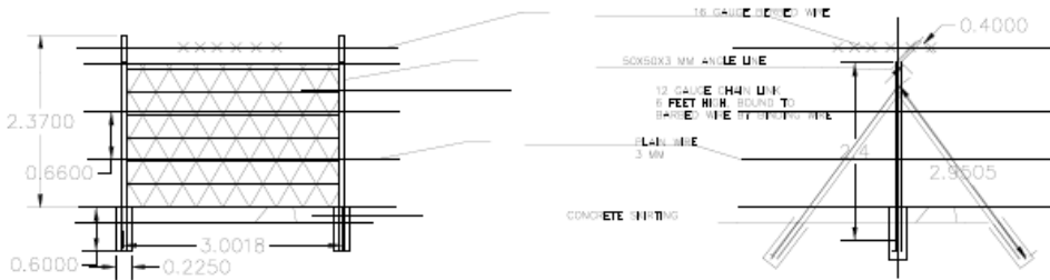
FENCE DETAIL FRONT VIEW
