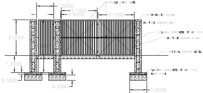
GATE DETAIL
