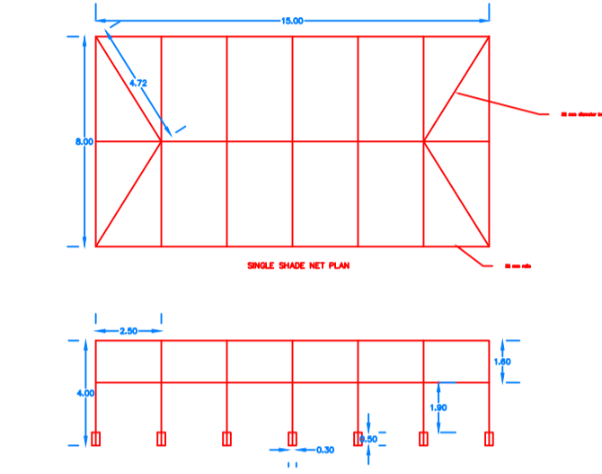
SINGLE SHADE SIDE VIEW
