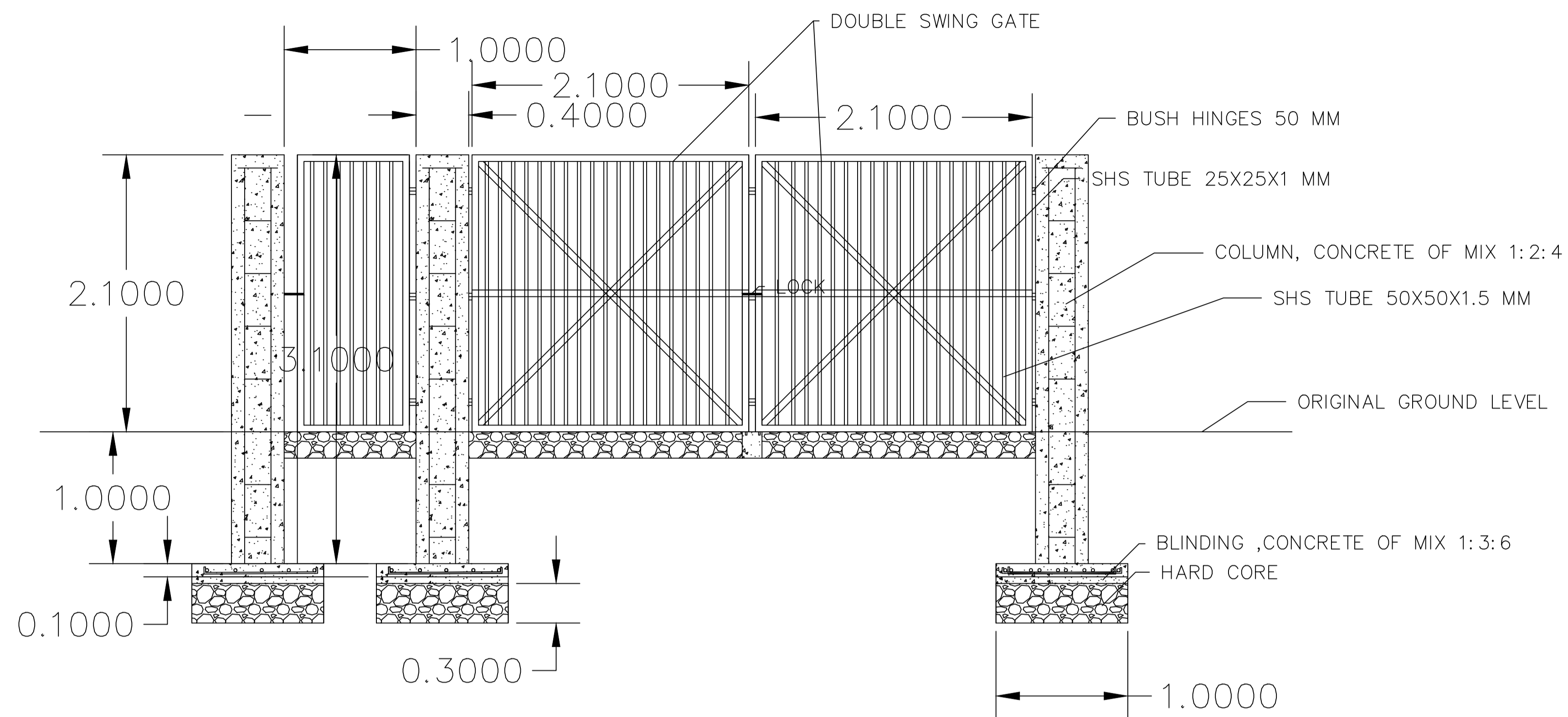
GATE DETAIL
