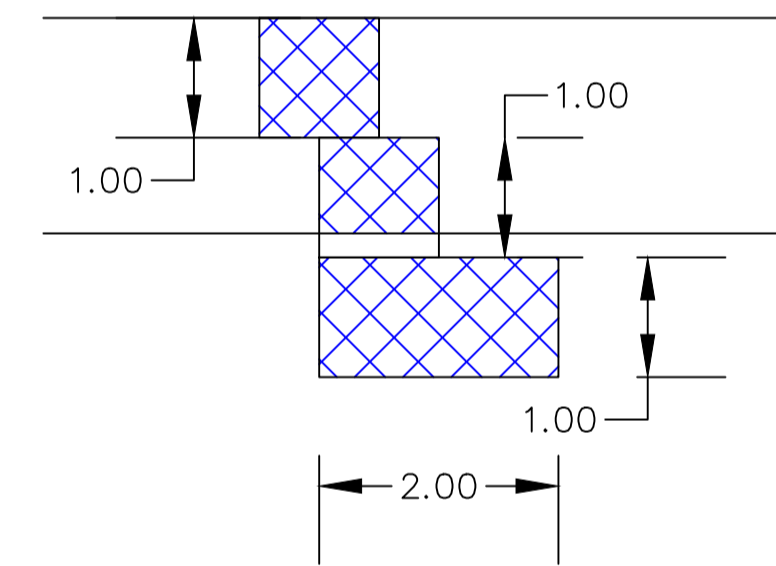
WEIR END VIEW
