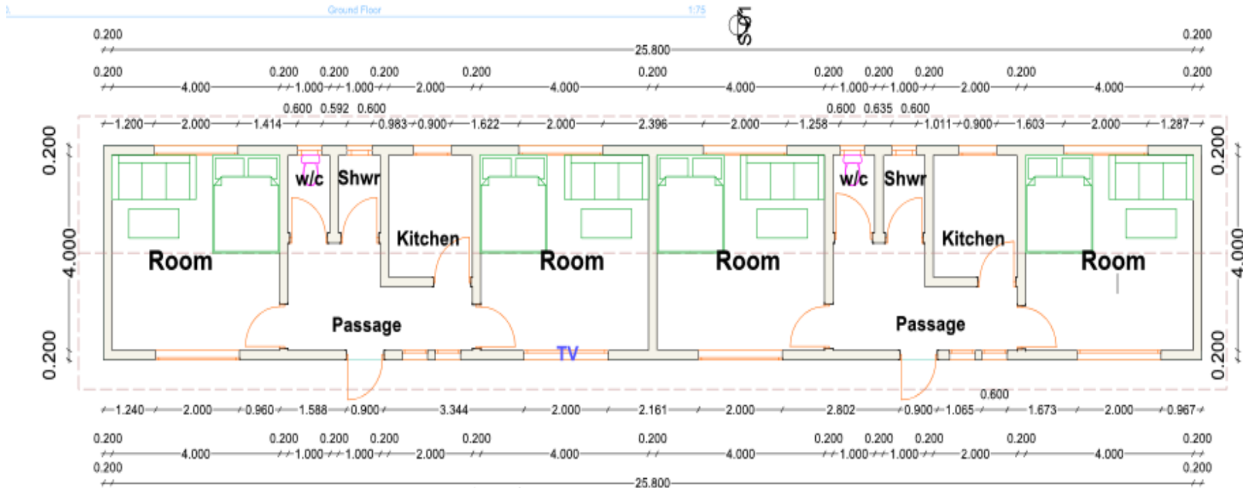
Ground floor plan 5
